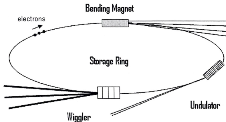
Figure 1. Schematic diagram of a storage ring and insertion devices - an undulator and a wiggler.
